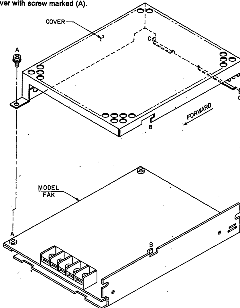
COVER INSTALLATION
